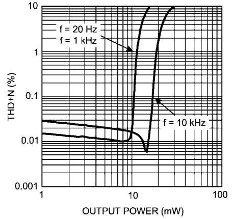
THD+N vs Output Power V_{DD} = 1.6V, R_L = 32\Omega, \text{One channel}
