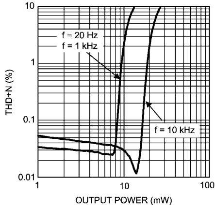
THD+N vs Output Power V_{DD} = 1.6V, R_L = 16\Omega, \text{One channel}
