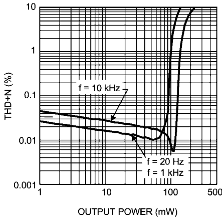
THD+N vs Output Power V_{DD} = 3V, R_L = 16\Omega, \text{One channel}
