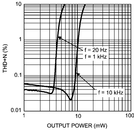
THD+N vs Output Power V_{DD} = 1.6V, R_L = 16\Omega, \text{Stereo}
