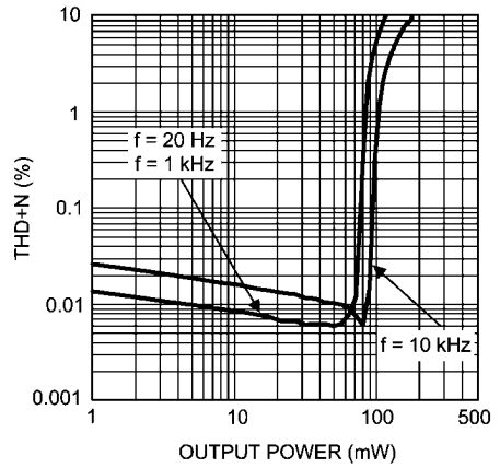
THD+N vs Output Power V_{DD} = 3V, R_L = 32\Omega, \text{One channel}
