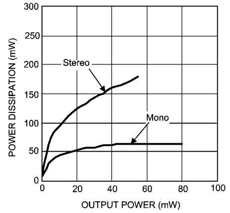
Power Dissipation vs Output Power V_{DD} = 3V, R_L = 32\Omega, f = 1kHz
