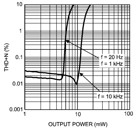
THD+N vs Output Power V_{DD} = 1.6V, R_L = 32\Omega, \text{Stereo}
